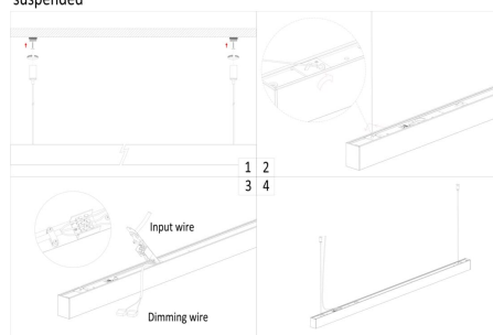
suspended
